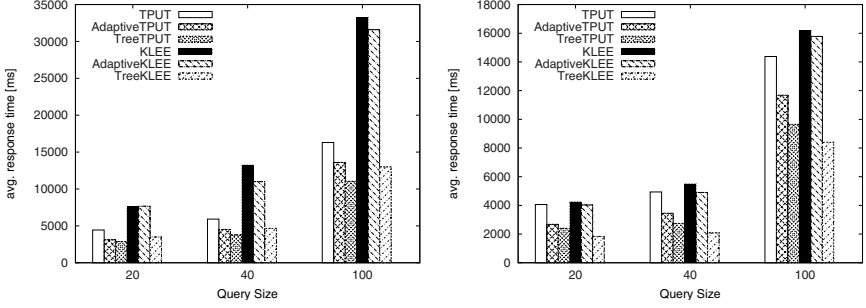
Fig. 4. Retail results in exact (left) and approximate (right) mode
