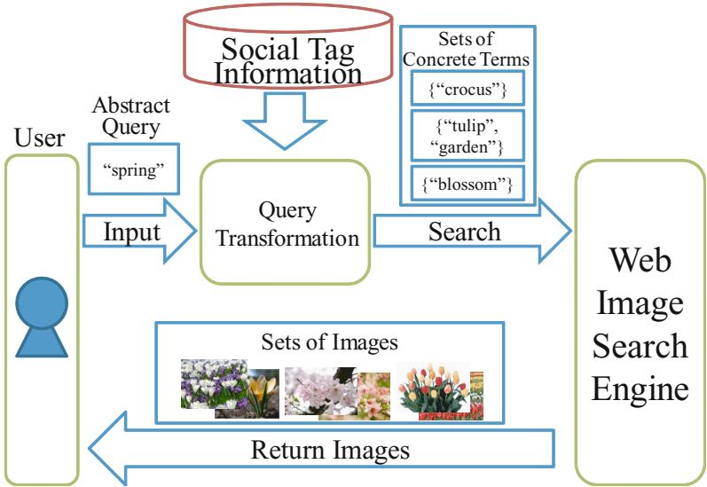
Fig. 4. Overview of our approach
