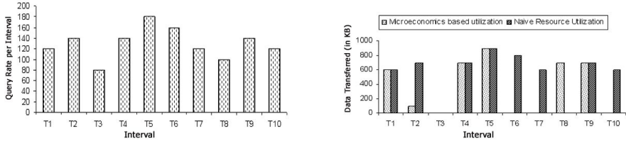
Fig. 7. Microeconomics Algorithm: (a) Server Workload; (b) Network Utilization
