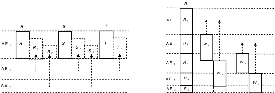
Fig. 3. (a) Remote Processing; (b) Fixed-size Window for Data Retrieval
