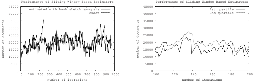
Fig. 2. Hash sketch based estimation of the number of documents under network churn
