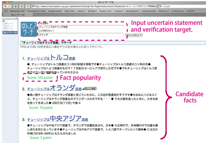
Fig. 1. System overview
