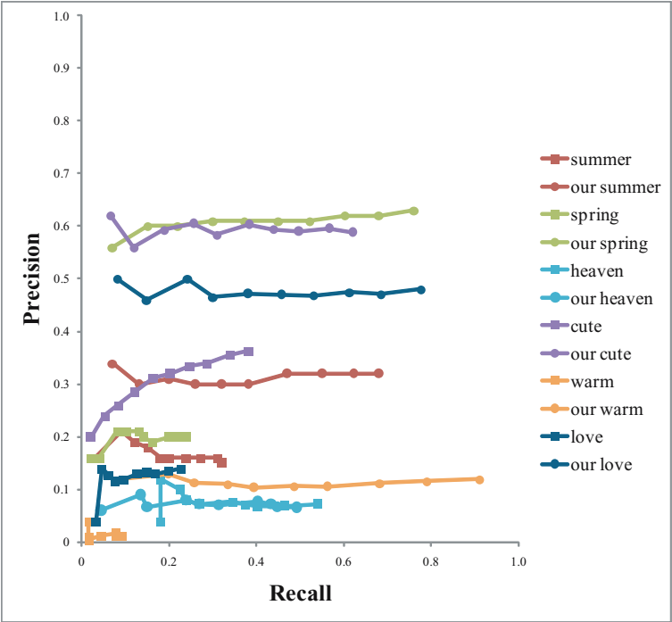
Fig. 7. Recall-precision curves for six abstract terms and corresponding sets of feature terms
