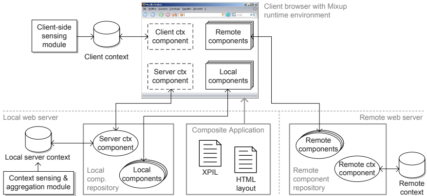
Fig. 3. The use of dedicated context components enables the development of context-aware web applications
