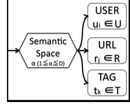
Fig. 3. Probabilistic Model
