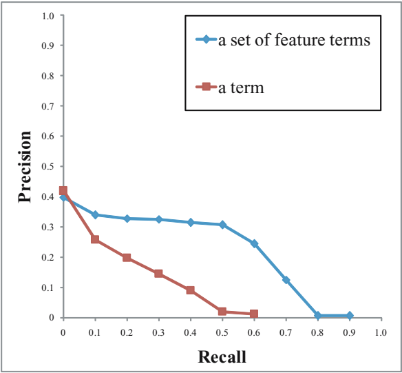
Fig. 6. 11-pt average precision for abstract terms and sets of feature terms
